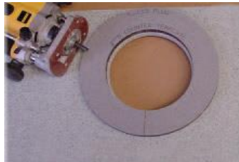
(2) Rout out damage with 1/2" straight bit/1" template guide
